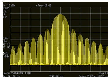
Add deep AM to the PSG for radar antenna test with scan modulation option HSM
